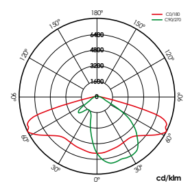
64 LEDS VA00K0M
