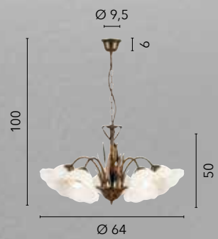
I-BYRON/5 RUG 8031440353045 5xE27
